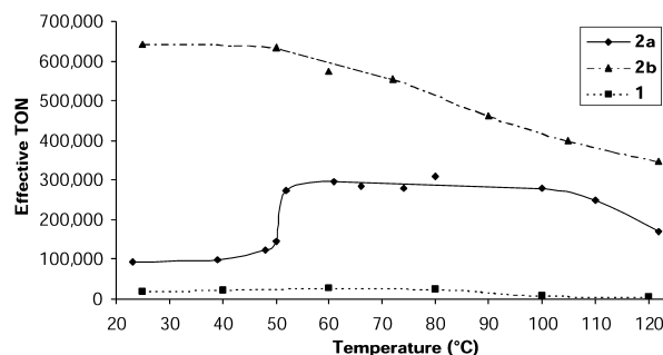
Figure 2. Effective TON as a function of temperature for catalysts 1 , 2a , and 2b for the metathesis of 1-octene. Reactions were deemed complete when no further metathesis activity was observed.
