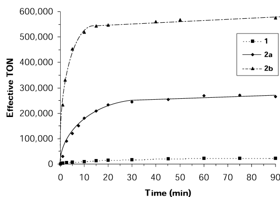
Figure 3. Effective TON as a function of time for catalysts 1 , 2a , and 2b in the metathesis of 1-octene at 60 °C, using 67,400, 718,000, and 1,154,000 equivalents of substrate, respectively.
