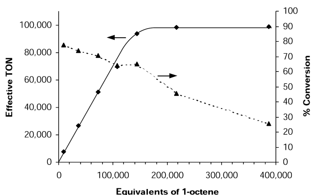
Figure 1. Effective TON and total conversion as a function of the number of equivalents of 1-octene for catalyst 2a at 22 °C.
